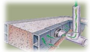
Vents Radon
