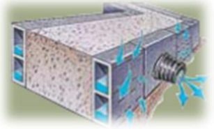
Drains Foundations
